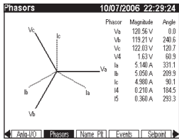
Phasors display
