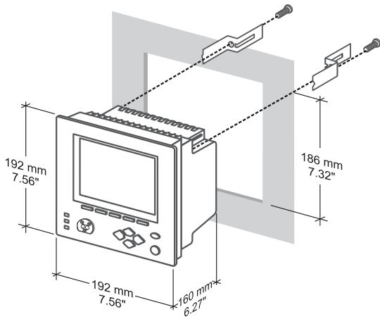
Meter installation showing rear mounting clips
